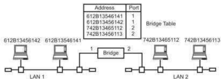
Figure A bridge connecting two separate LANs
